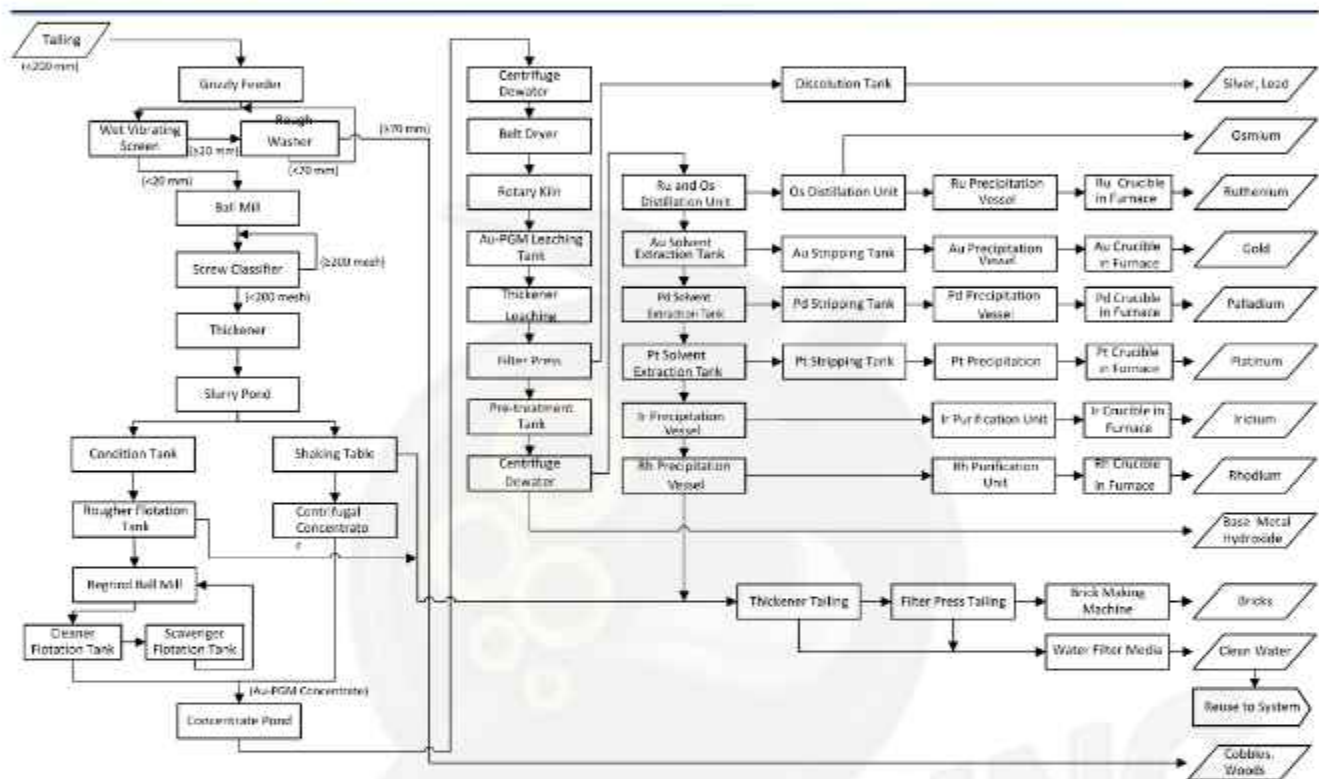
Process Flow Diagram Au-PGM EXTRACTION - Possible Routes.
